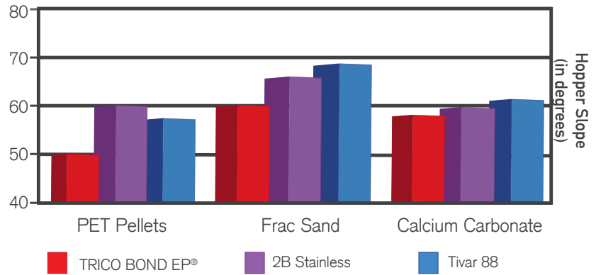
Hopper Slope Required for Mass Flow (product tested at 72°F)
